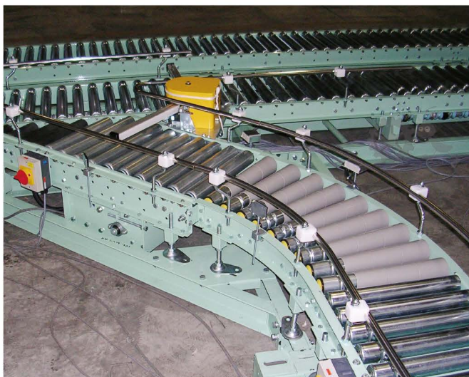
转弯滚筒输送机应用图 Application picture of curved roller conveyor
