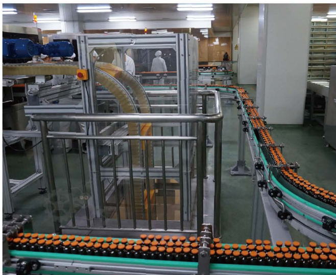
柔性夹持提升机应用图 Application picture of gripper Conveyor
